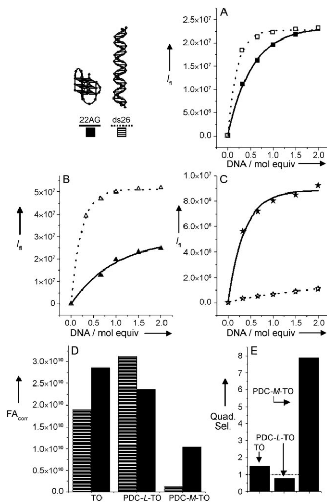
Figure 1. A–C) Fluorescence response of TO (A), PDC- L -TO 1 (B), and PDC- M -TO 2 (C, 1 \mu M in 10 mM lithium cacodylate buffer, 1 mM KCl, \lambda_{\text{ex}} = 490 (A, B) and 500 nm (C)) upon addition of increasing amounts (0–2 \mu M) of quadruplex DNA (22AG, solid line) or duplex DNA (ds26, dotted line). D) Fluorescence areas (corrected with regards to absorbance ( FA_{\text{corr}} ), see the Supporting Information) of TO, PDC- L -TO 1 , and PDC- M -TO 2 upon addition of 2 equiv of 22AG (black bar) or ds26 (striped bar). E) Quadruplex/duplex DNA fluorescence selectivity of dyes (normalized at 1 for ds26 fluorescence). I_f : fluorescence intensity, Quad. Sel.: quadruplex selectivity.
