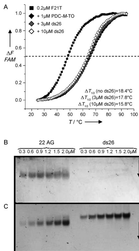
Figure 2. Selectivity of PDC-M-TO 2 . A) FRET melting curves for experiments carried out with F21T (0.2 \mu\text{M} in 10 mM lithium cacodylate buffer, 100 mM NaCl (black square)) with PDC-M-TO 2 (1 \mu\text{M} ) in the absence (black diamond) or presence of competitive ds26 (3 \mu\text{M} (gray diamond) and 10 \mu\text{M} (white diamond)). B,C) Gel electrophoresis (20% acrylamide, in 1 \times TBE buffer + 20 mM KCl, 5 ^{\circ}\text{C} ) of DNA (22AG (left lanes) and ds26 (right lanes) at concentrations from 0.3 to 2.0 \mu\text{M} stained by PDC-M-TO 2 (B, 5 \mu\text{M} , 5 h) and post-stained by PDC-L-TO 1 (C, 2 \mu\text{M} , 1 h) ( \lambda_{\text{ex}} = 532 nm, \lambda_{\text{em}} = 550 nm). \Delta F_{\text{FAM}} : normalized FAM fluorescence.
